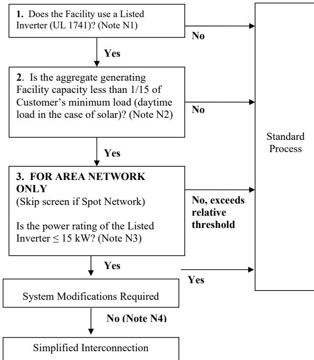
Figure 2 – Simplified Interconnection to Networks
