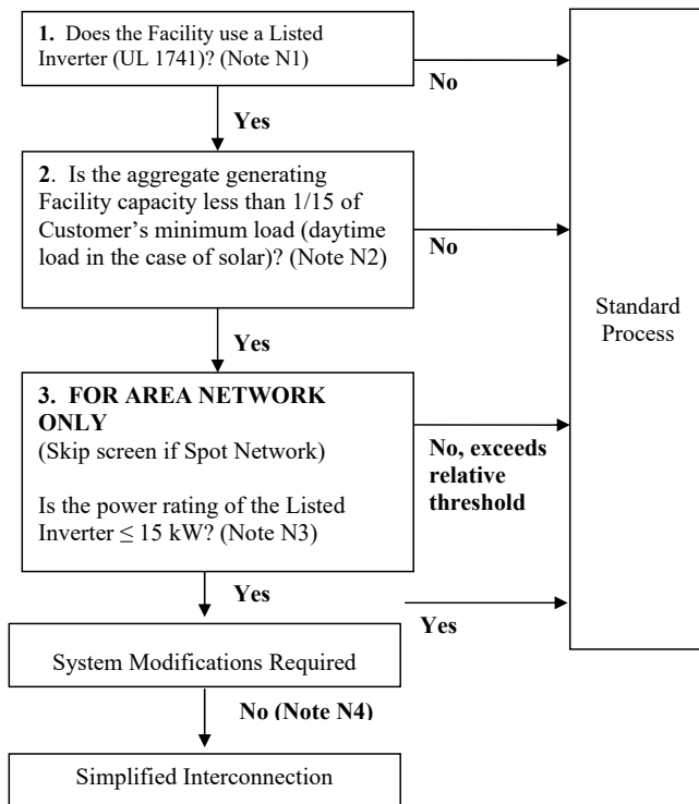
Figure 2 – Simplified Interconnection to Networks
