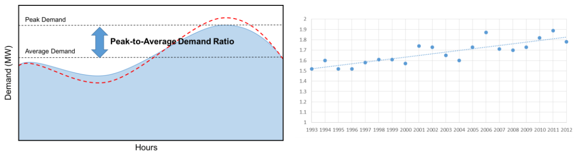
Figure 2-7: Peak-to-Average Demand Ratio Illustration and ISO-NE Annual Increase (1993-2012) 44
