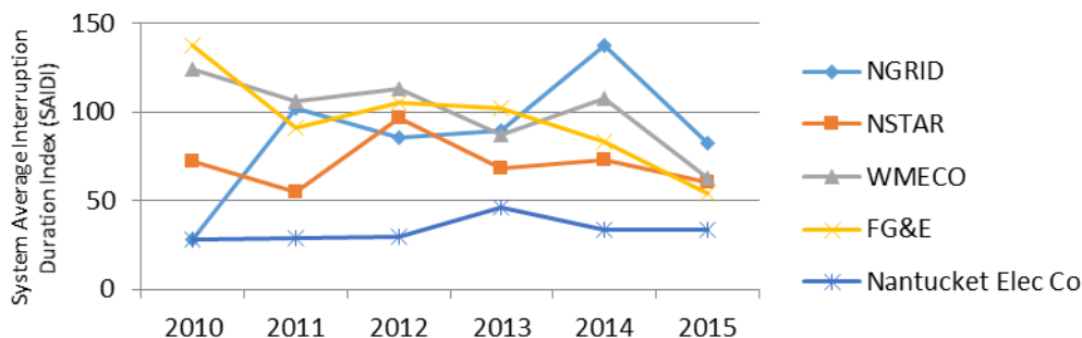
SAIDI for Massachusetts Utilities (2010-2015)
