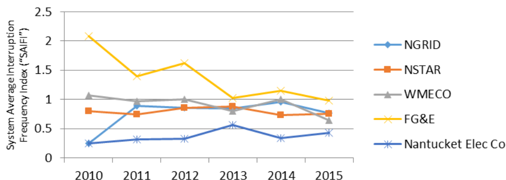
Figure 2-17: Reliability Metrics (SAIDI/SAIFI) for Massachusetts Utilities (2010-2015) 71
