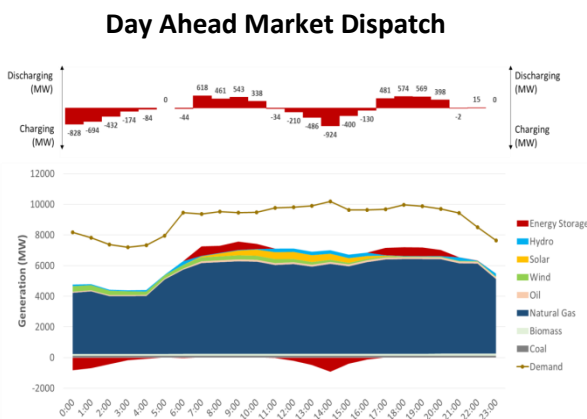
Figure 4-21: Hourly Market Operations with Energy Storage
