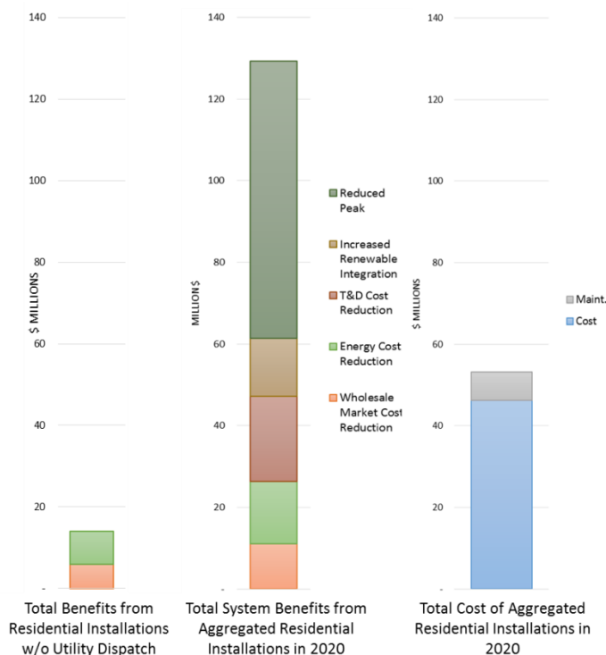
Figure 5-10: System Benefits Analysis for Behind-the-Meter Residential Energy Storage Project Dispatched by Local Utilities
