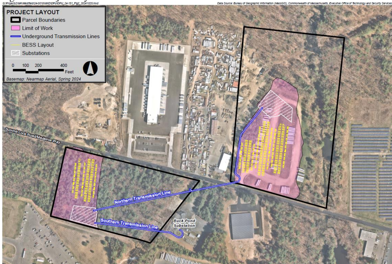
Figure 2: Project Layout.
