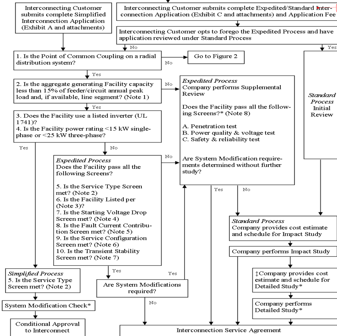
Figure 1 – Schematic of Massachusetts DG Interconnection Process
